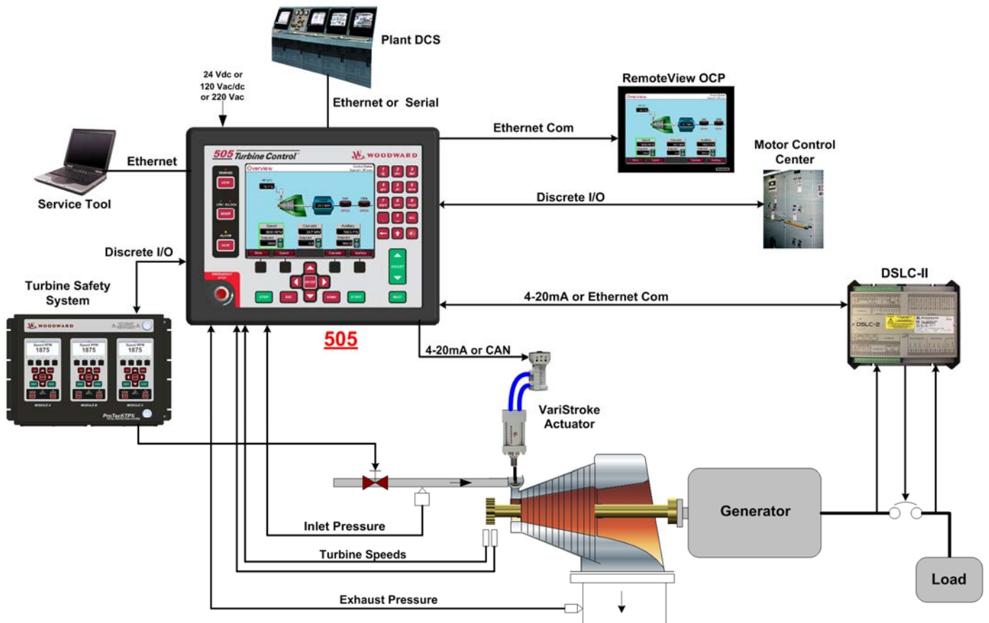
Figure 3. Typical 505 Application
